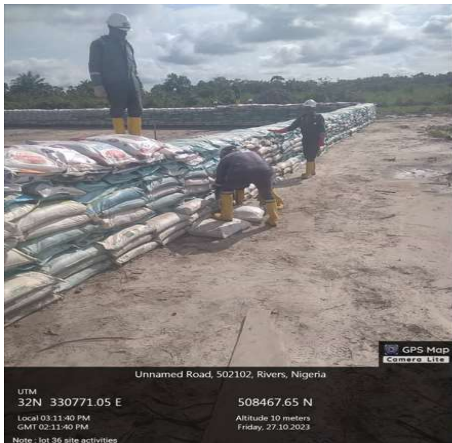
Plate 7: Cross Section of Stacked Sandbags
